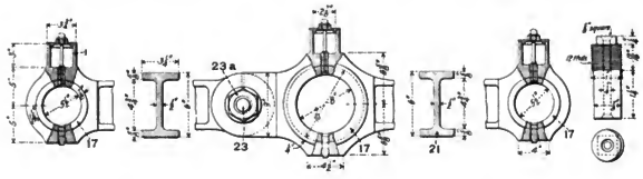
Figs. 1157-1158. Side Rods for Atlantic (4-4-2) Locomotive. P. R. R.
